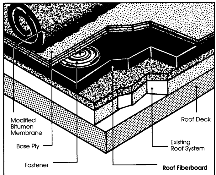
FIG B - Typical Modified Application
