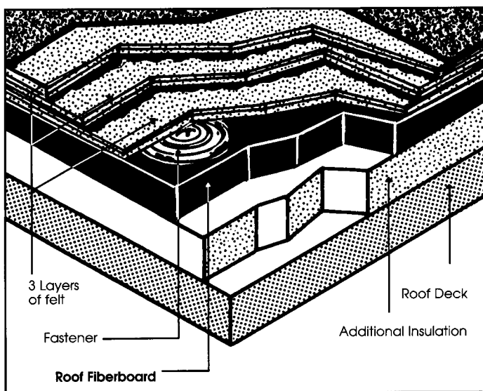
FIG A - Typical Built-Up Roof Application
