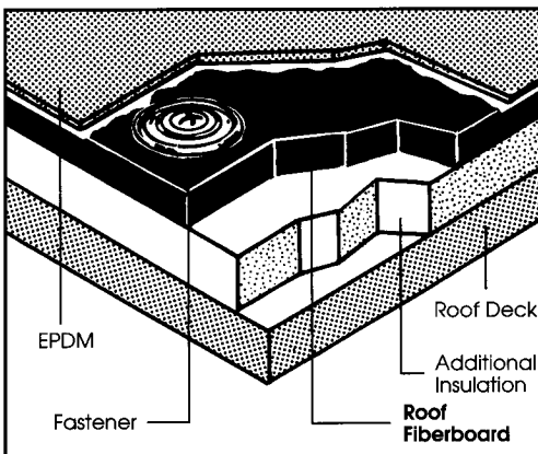
FIG C - Typical Membrane Application
